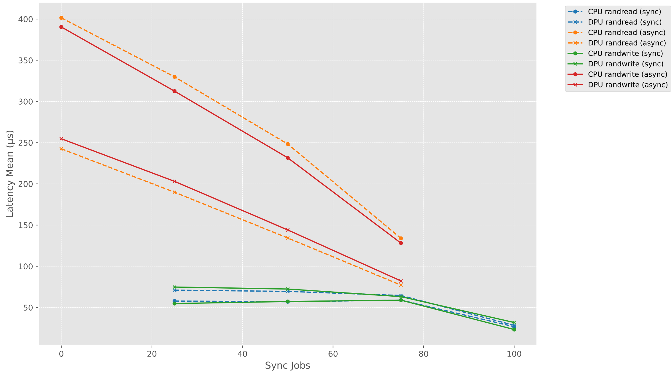
Latency Mean vs Sync Jobs (mixed) - RAND (CPU vs DPU)
